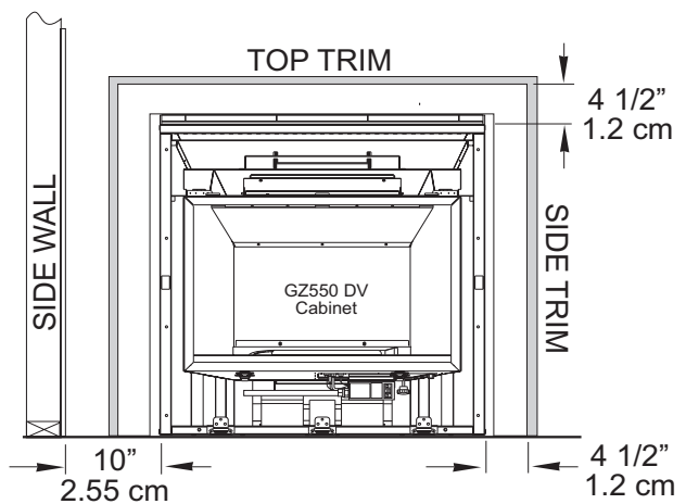
Figure 8. Minimum Wall and Trim Clearance. Measured from the cabinet, not standoffs or cast iron panels. Maximum Top & Side Trim depth: 2 1/2" (64 mm)
