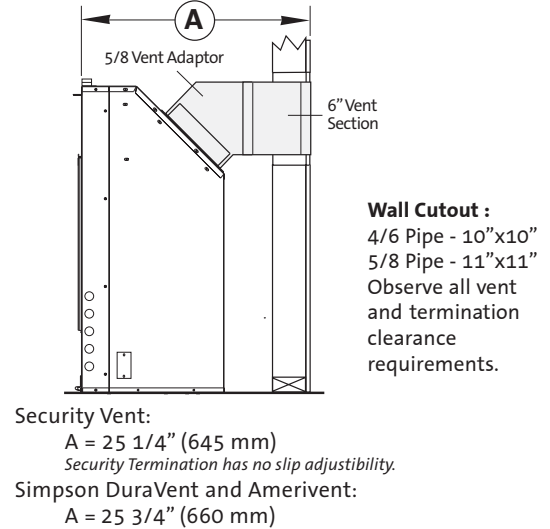
Figure 2. Minimum horizontal vent allowance through wall.
