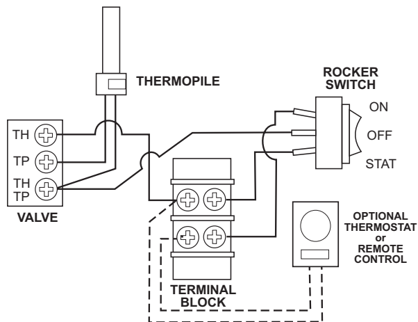
Figure 36. GZ 550 DV II Acadia Wiring Diagram.
