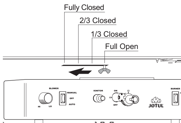
Figure 19. Vent restrictor adjustment.
