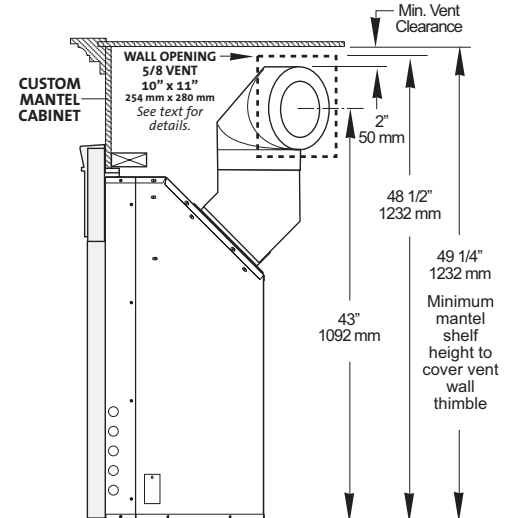
Figure 5a. Corner Installation - 5/8 vent, rear termination.
