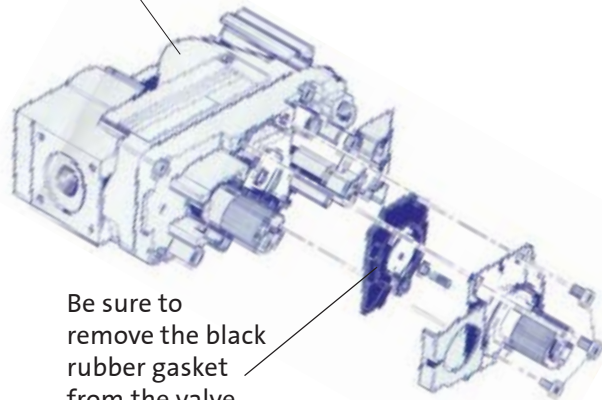
Figure 34. Valve Regulator replacement.
