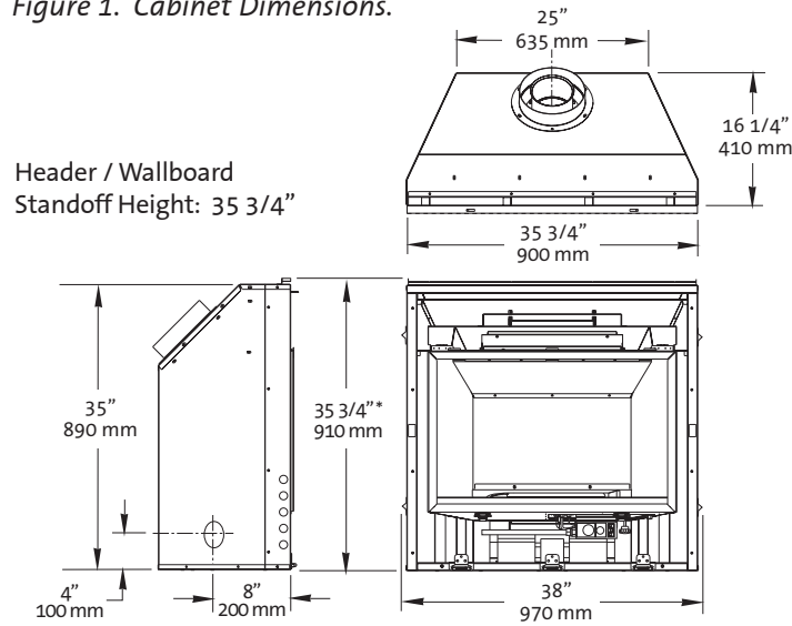
Figure 1. Cabinet Dimensions.
