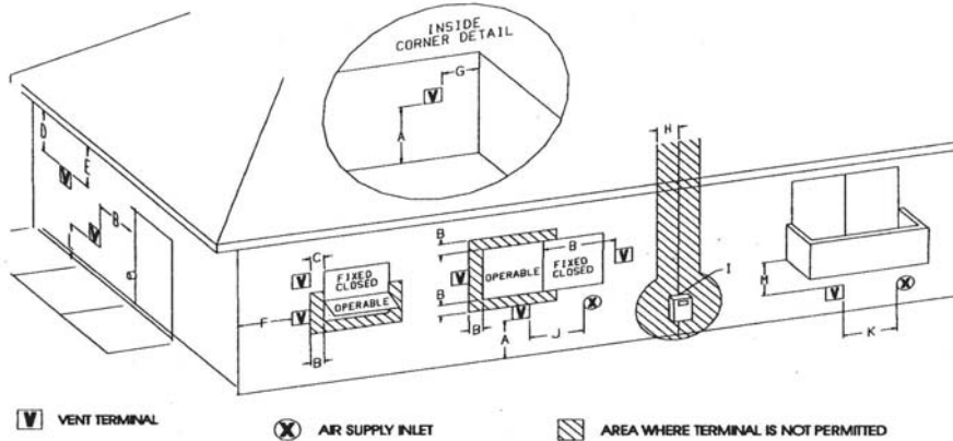
Figure 17. Vent Terminal Clearances.
