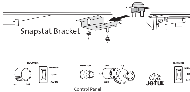
Figure 22. Install snapstat bracket and switch box.
