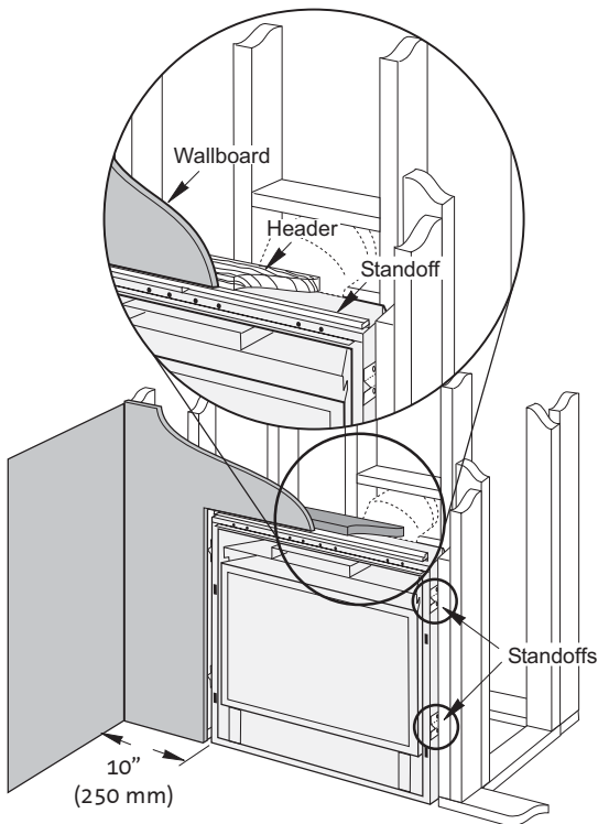
Figure 6. Header and Side Standoffs
