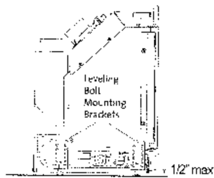
Figure 37. The leveling bolts should not be extended further than 1/2 ".
