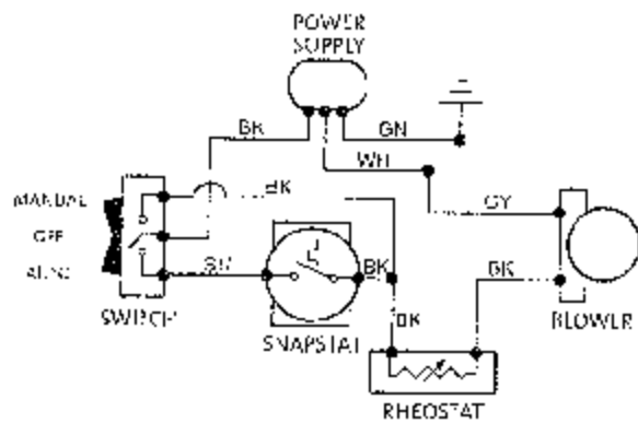
Figure 19. Blower Wiring Diagram - G1450 Katahdin
