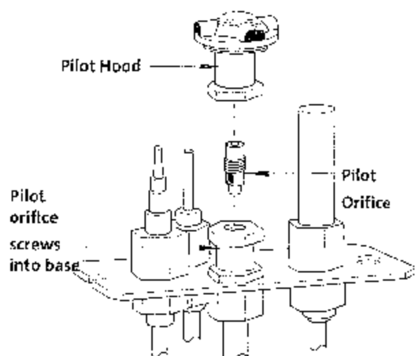
Figure 9. Pilot Assembly.
