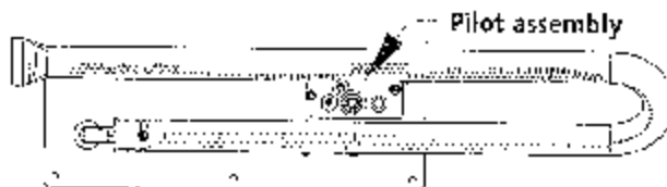
Figure 29. Pilot assembly location.
