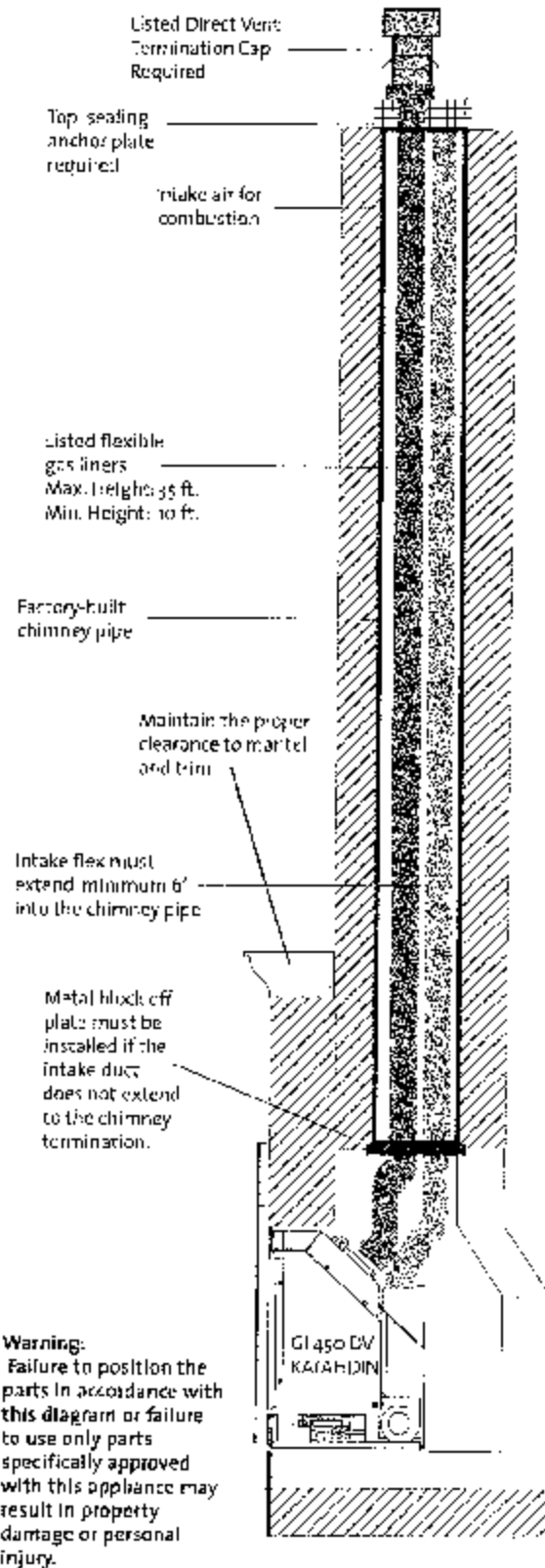
Figure 4. Venting through prefabricated fireplace chimney.
