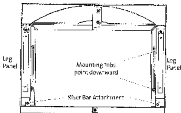
Figure 25. Surround mounting tab locations.
