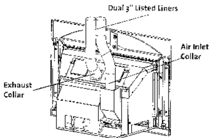
Figure 3. Duct collar locations.
