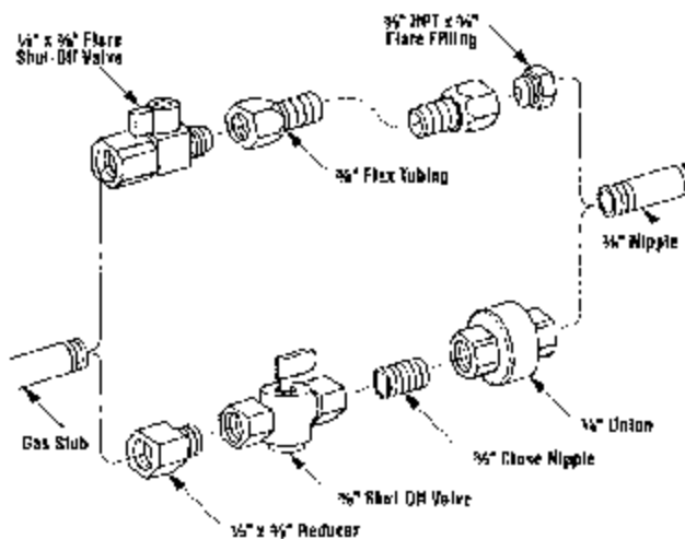
Figure 12 Gas connection components.
