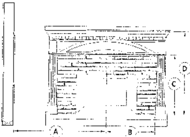
Figure 5. Fireplace clearances to combustible materials.
