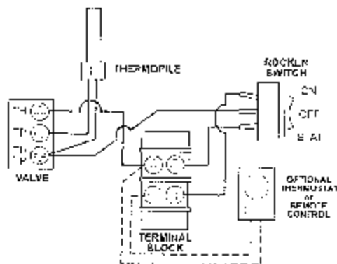
Figure 20. Wiring diagram / G1450 DV Katahdin
