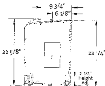
Figure 2. Firebox dimensions.
