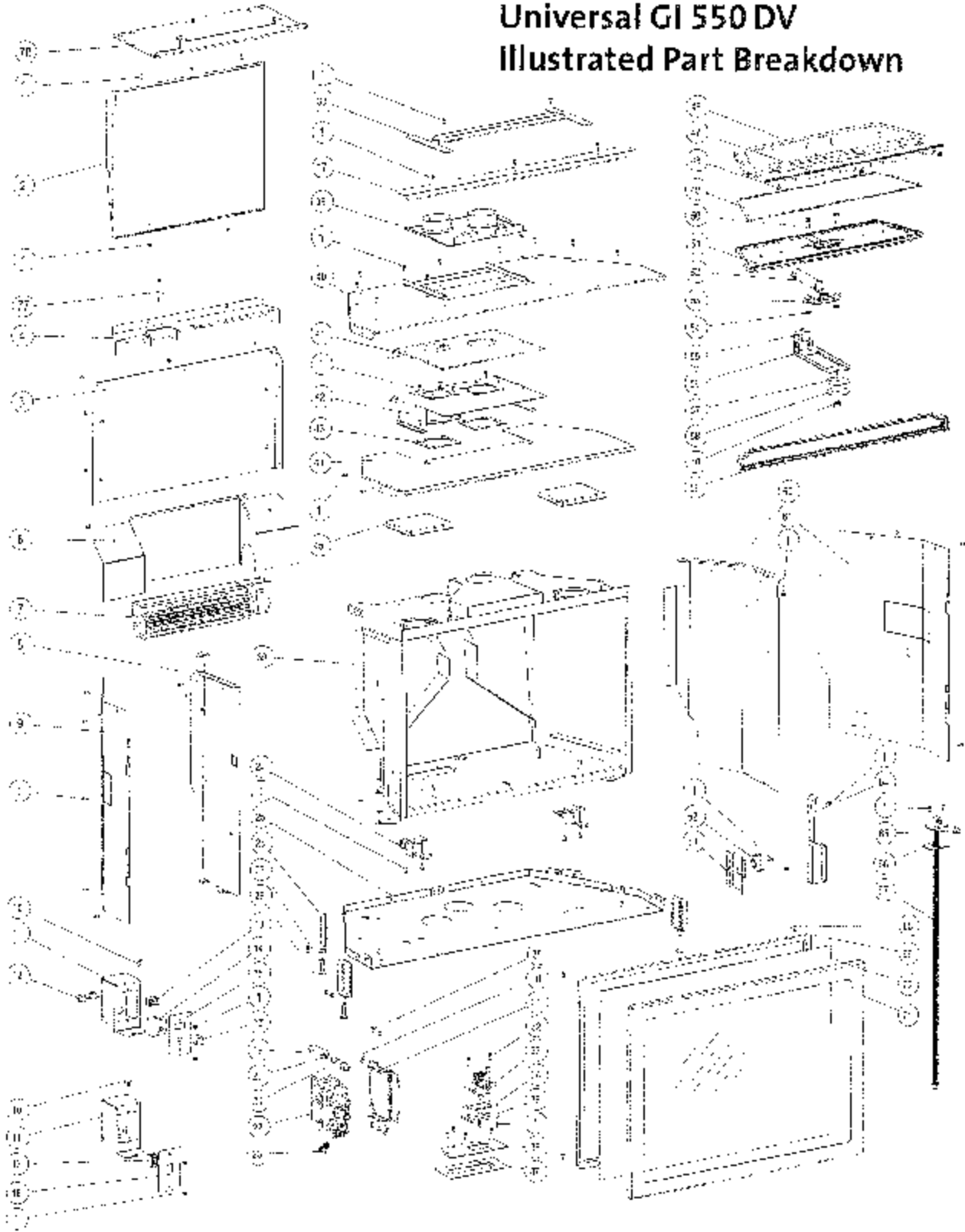
Figure 37. Part Identification.
