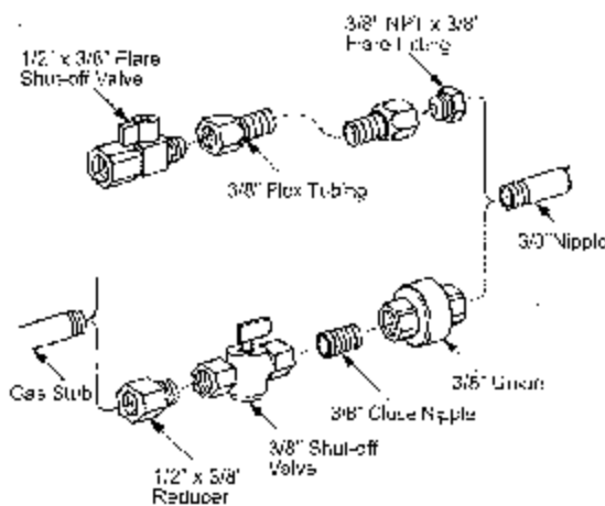
Figure 11. Gas supply line fittings.
