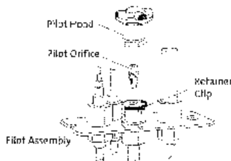
Figure 16. Pilot Orifice replacement.
