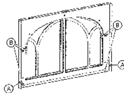
Figure 46. Rear view of door frame.
