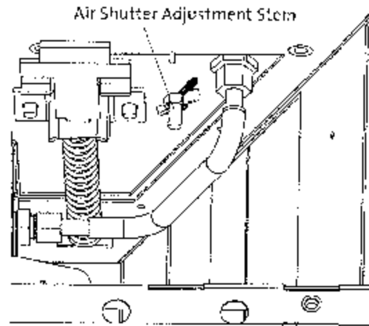
Figure 49. Air Shutter adjustment location.
