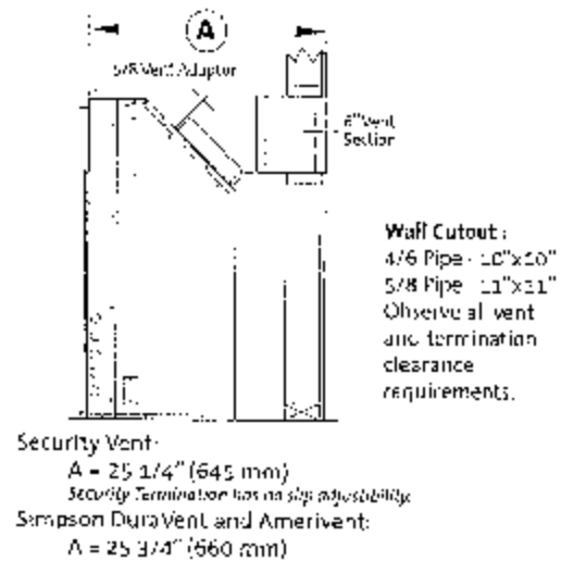
Figure 2. Minimum horizontal vent allowance through wall.
