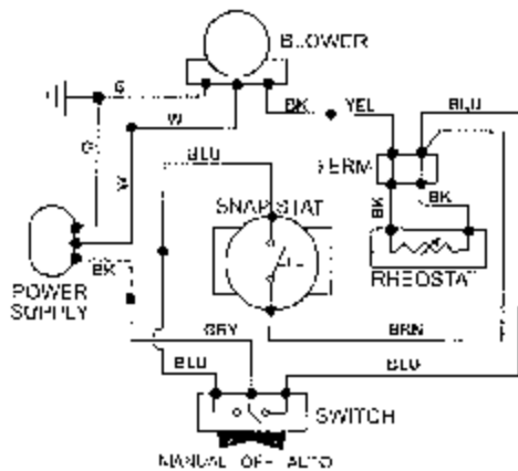
Figure 54. ZGS50 DV Acadia Blower Wiring Diagram
