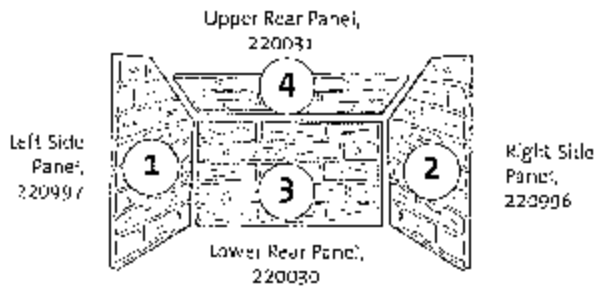
Figure 37. Panel installation order.
