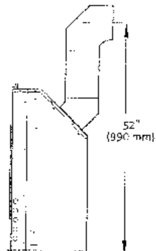
Figure 14. Minimum centerline for horizontal termination of 4/6 pipe
