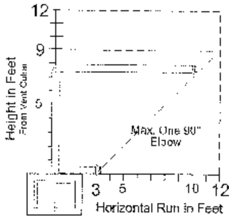
Figure 15. Horizontal termination - 5/8 pipe.
