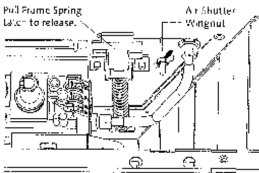
Figure 29. Frame latch and air shutter stem location.
