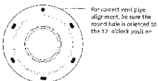
Figure 23. 4/6 Vent Collar orientation.
