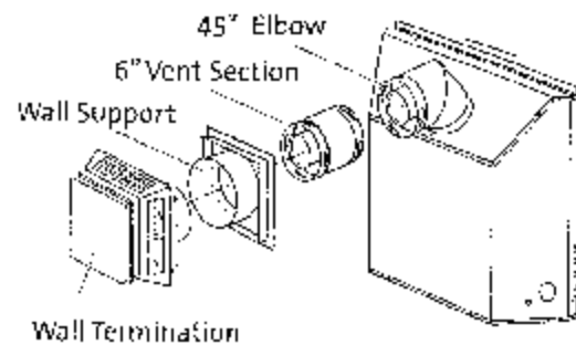
Figure 11. Typical minimum horizontal vent configuration - 5/8 Simpson DuraVent. Do not use 4/6 pipe in this configuration.
