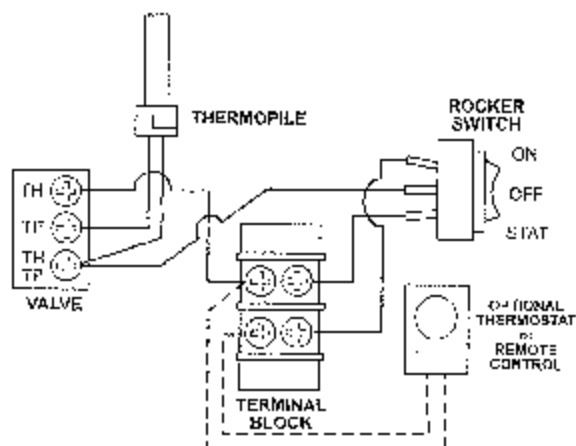
Figure 36. ZG550 Acadia Wiring Diagram
