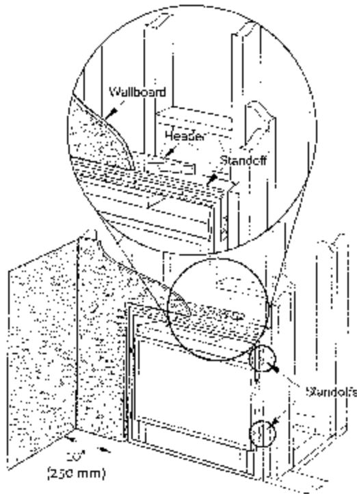
Figure 6. Header and Side Standoffs
