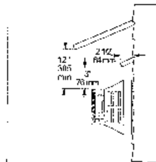
Figure 18. Wall Vent Terminal / Clearances to Overhangs
