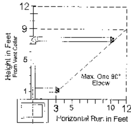
Figure 16. Horizontal Termination - 4/6 Pipe. Minimum 1 ft rise required.
