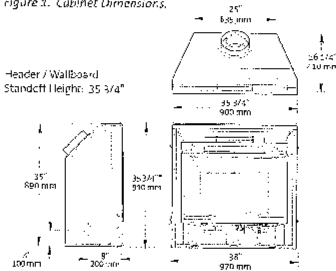
Figure 1. Cabinet Dimensions.
