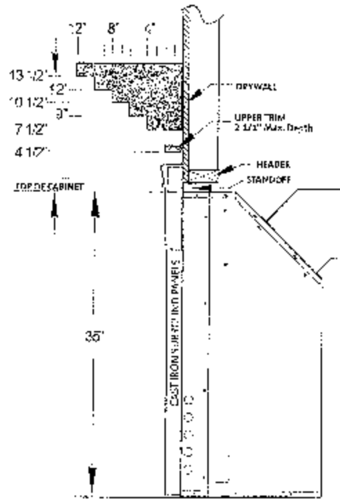
Figure 7. Minimum Mantel Clearances. Measure clearances from the top of the fireplace cabinet before installation of the cast iron surround panels.
