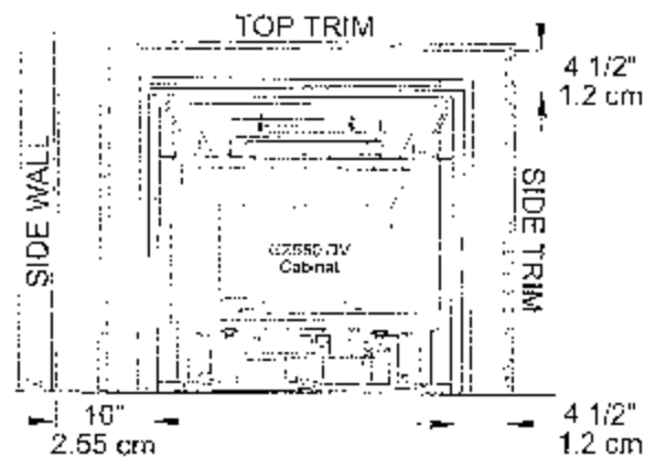
Figure 8. Minimum Wall and Trim Clearance. Measured from the cabinet, not standoffs or cast iron panels. Maximum Top & Side Trim depth: 2 1/2" (64 mm)
