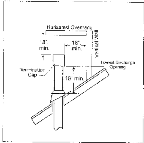
Figure 10. Gas Vent Height Rule: Vertical vent termination height above roof.
